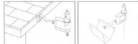
Figure 6: Attaching sensor/transmitter to gutter or flat surface
